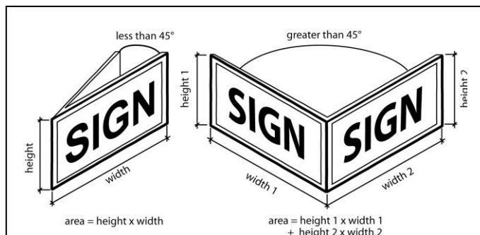
Figure 19.8.12-B: MULTI-SIDED SIGN FACE AREA CALCULATION
